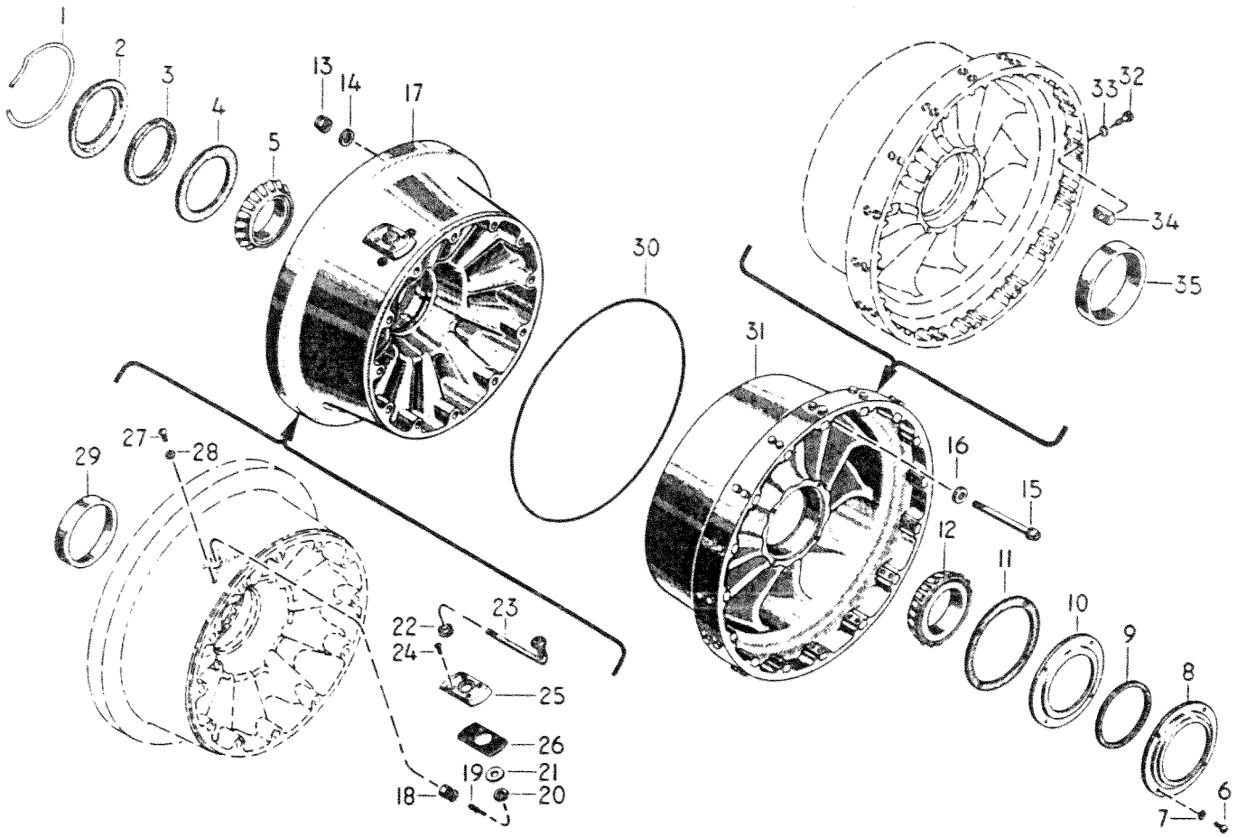
Figure 17.00-20 MW4 — MAIN WHEEL Assembly No. 9541085
